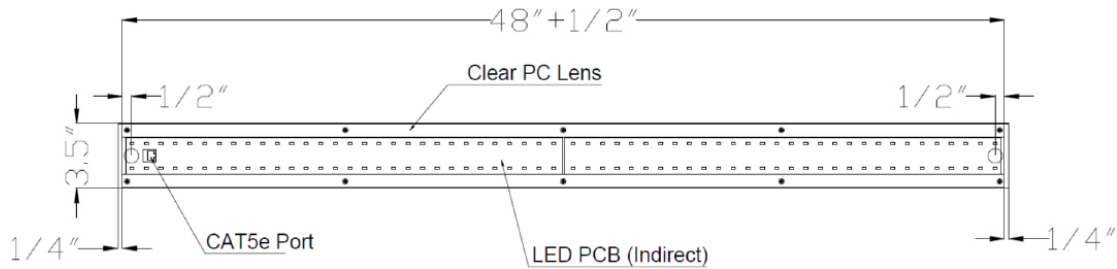
MHTL-CUBE-L-4FT Suspended Side View
