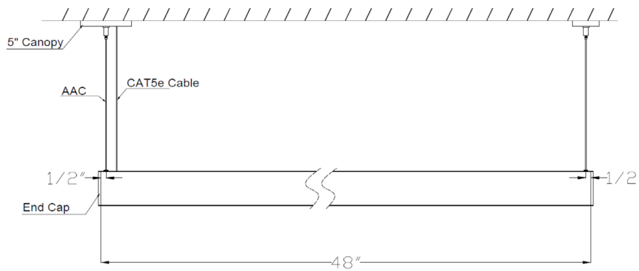
MHTL-CUBE-L-4FT Suspended Side View
